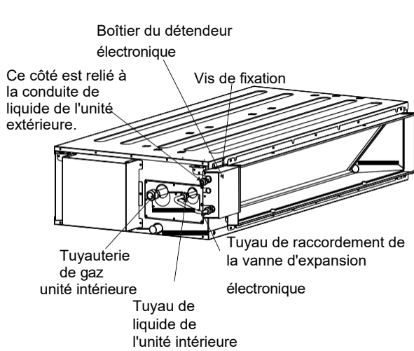
Figure 5.6 Pression statique standard et gainable haute pression 7.1kW~9.0kW
