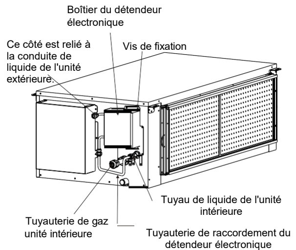
Figure 5.7 Pression statique standard et gainable haute pression 10.0kW
