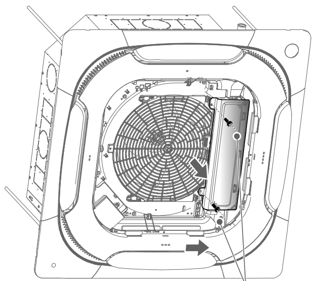
Screw (two)
